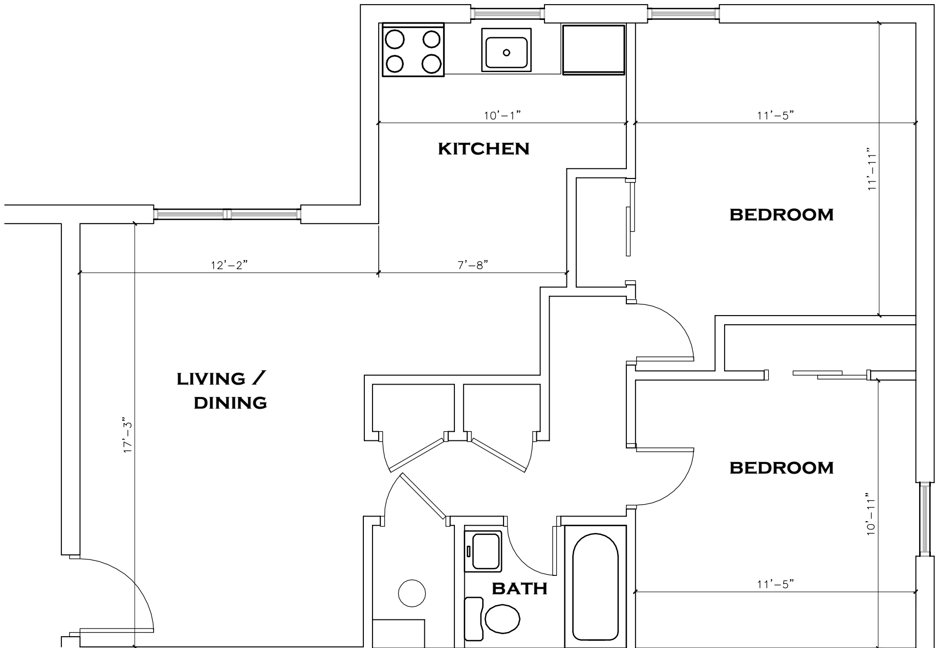
LINCOLN CROSSING - APARTMENT B9 - 766 SF
